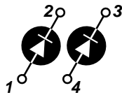
Parallel APT2X101D120J
